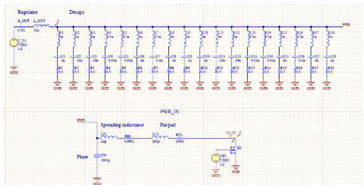
Example SPICE model generated in Altium Designer. This model includes a decoupling capacitor bank, equivalent circuits for planes, and a simple switch to simulate current draw by an integrated circuit.
