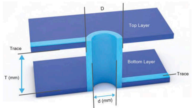
Fig. 5. Via dimensions
