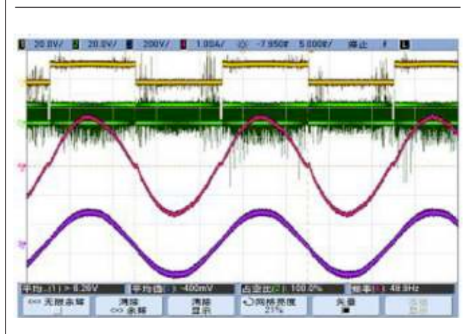
(Figure 1: Circuit diagram of an solar inverter and its current waveform)
