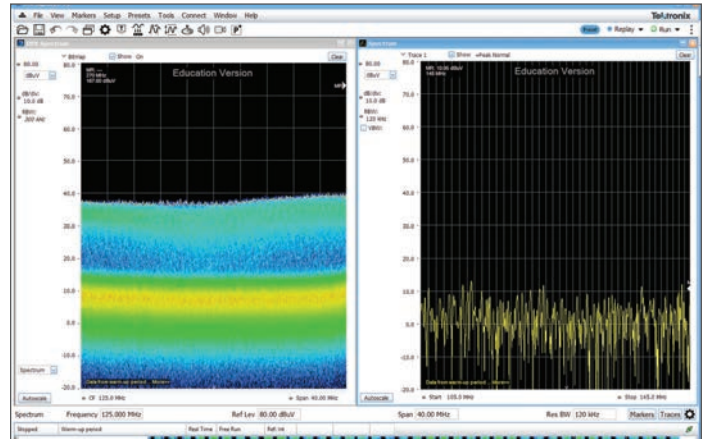
Figure 4 - Broadband emissions from the DC-DC converter looking from 105 to 145 MHz. The swept measurement on the right was unable to successfully capture this, except for an occasional burst. Max Hold mode would have helped, but would have taken at least a minute to "fill in" the display. But once the display was filled in, you may not have been able to see the following two very different modes in Figures 5 and 6.
