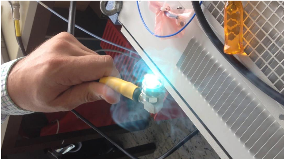
Figure 11 - Amplifier continuing to deliver power to an open load
