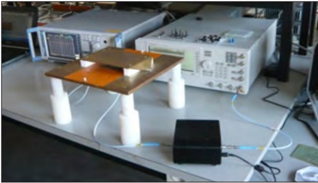
FIGURE 15: Stripline fixture.
