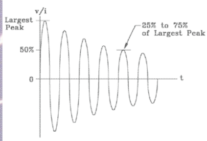
Figure 22-4 Voltage/Current Waveform 3
